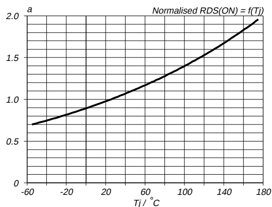
Fig.9. Normalised drain-source on-state resistance. a = R_{DS(ON)}/R_{DS(ON)25^\circ \text{C}} = f(T_j) ; I_D = 20 \text{ A} ; V_{GS} = 5 \text{ V}
