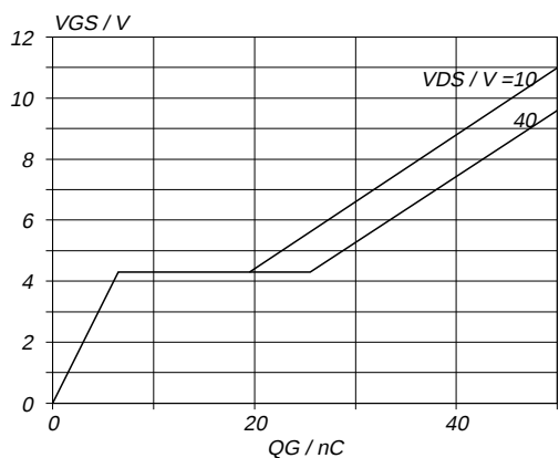
Fig.13. Typical turn-on gate-charge characteristics. V_{GS} = f(Q_G) ; conditions: I_D = 39\text{ A} ; parameter V_{DS}
