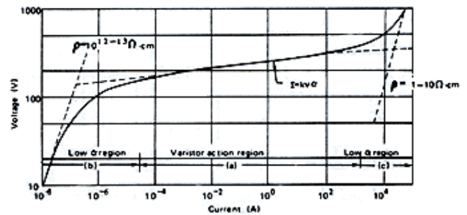
Typical Varistor V - I Curve
