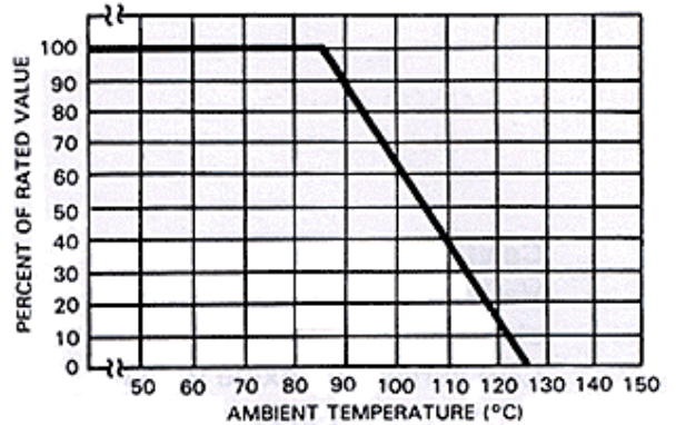
Current, Energy and Power Derating Curve
