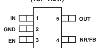
DCQ PACKAGE SOT223 (TOP VIEW)
